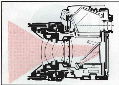
Full-field integral exposure metering
