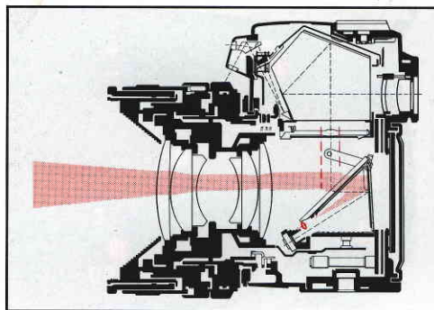
Selective exposure metering
